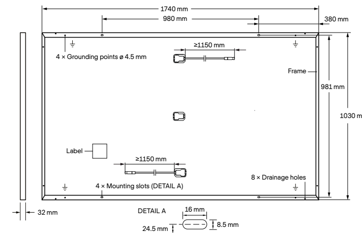
Fig. 1: External dimensions and components for Q.PEAK DUO-G6, Q.PEAK DUO-G6+, Q.PEAK DUO BLK-G6 and Q.PEAK DUO BLK-G6+
