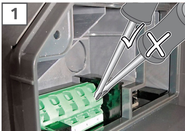
Fig. 2-1: Power supply terminal
