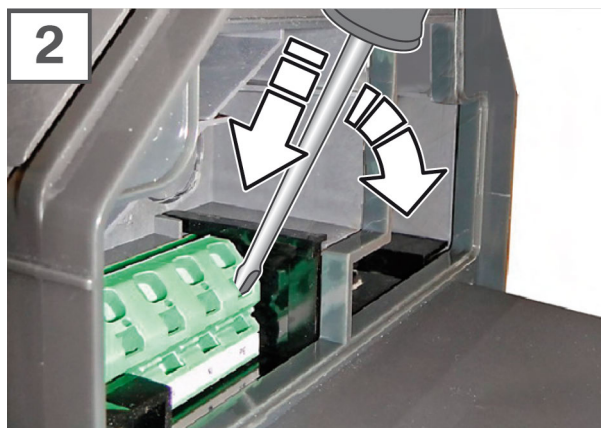
Fig. 2-2: Opening the power supply terminal
